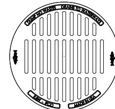
1848 Type M Grate Approx 126 sq. in. open area "DUMP NO WASTE!" lettering
